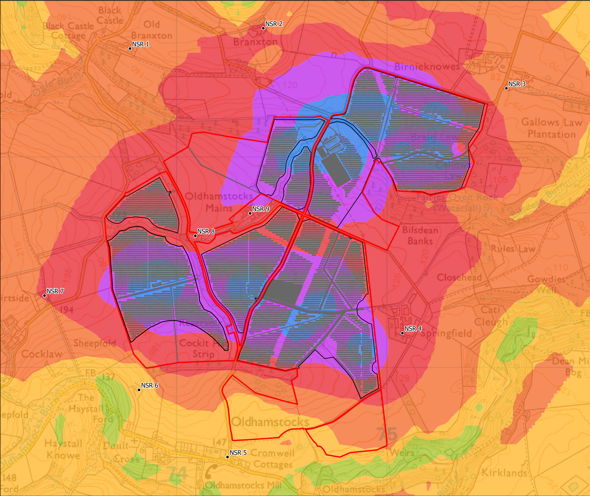
Springfield Solar Farm and BESS Figure 12.2 Unmitigated Operational Noise Modelling Contours (Day & Night) (4m above Ground)
